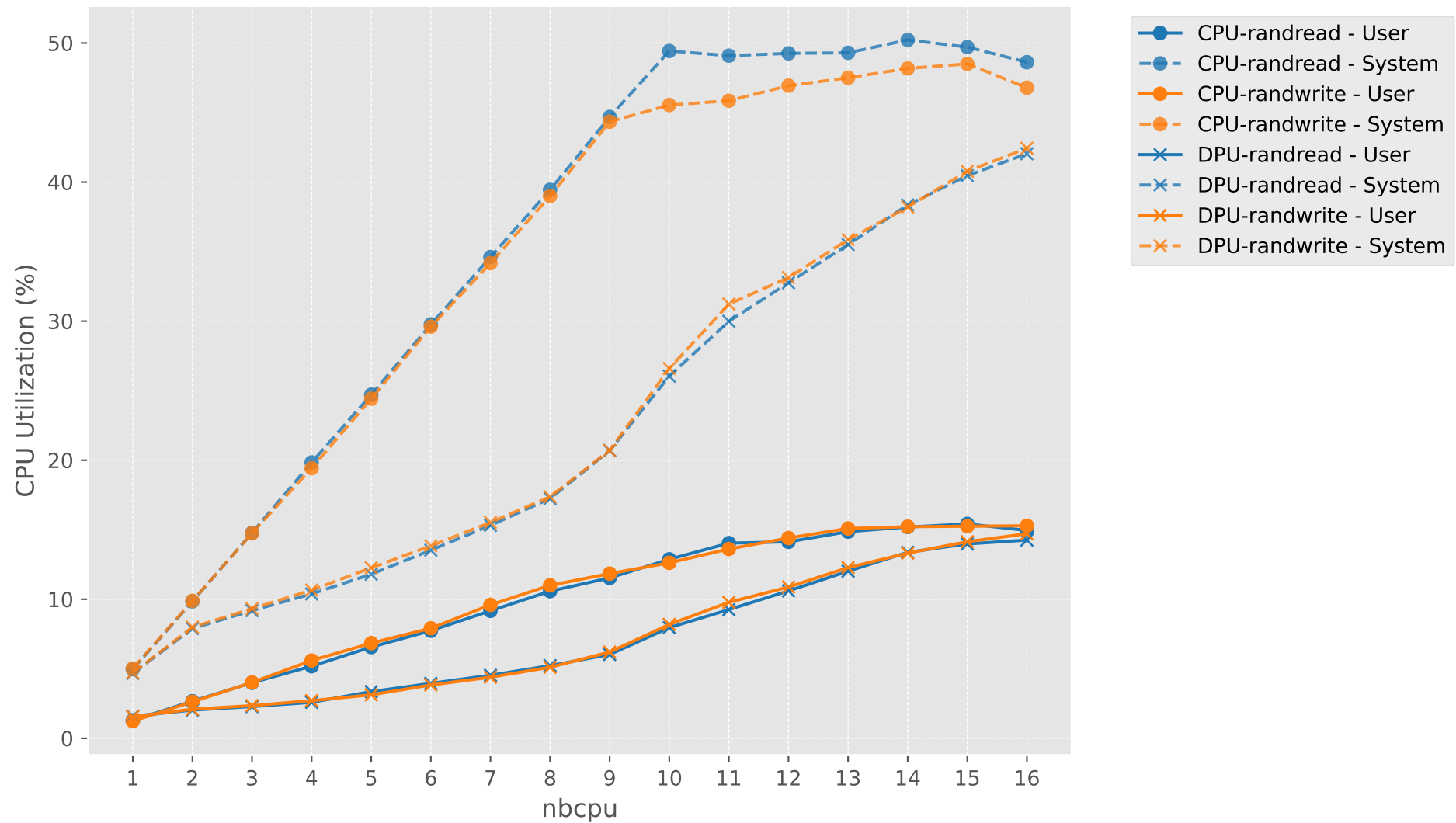
CPU Utilization vs nbcpu
